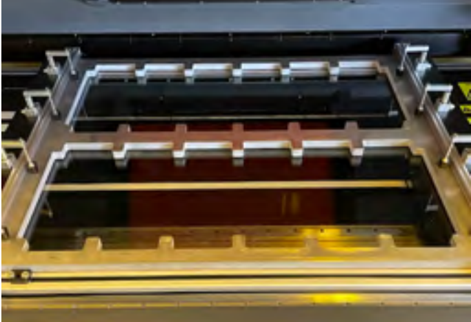
In addition to standard single frames, the LTS 6080 is compatible with frame holders for many small screens.
