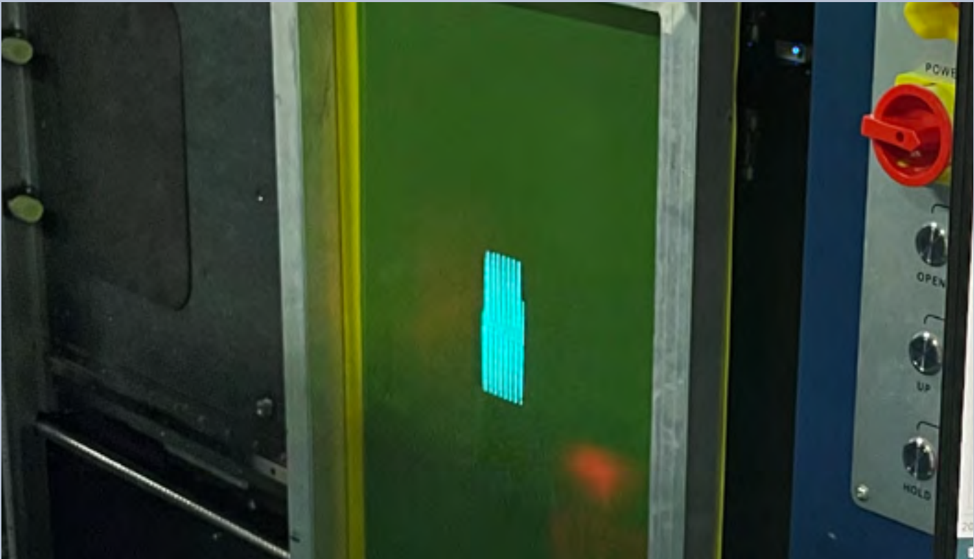
96 Laser Matrix scans while the screen steps across the image area
